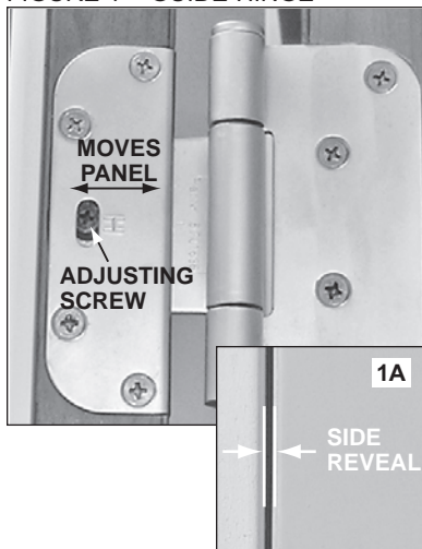
FIGURE 1 – GUIDE HINGE
